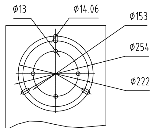
Arrester Bracket Drill Pattern
