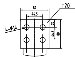
HV Bushing Terminal(COPPER)
