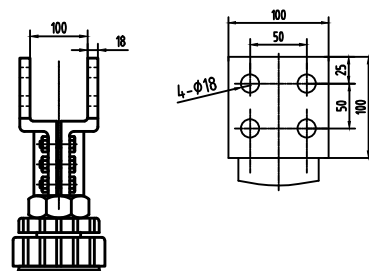
LV Bushing Terminal(COPPER)
