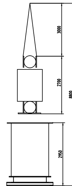
Core and coil lifting
